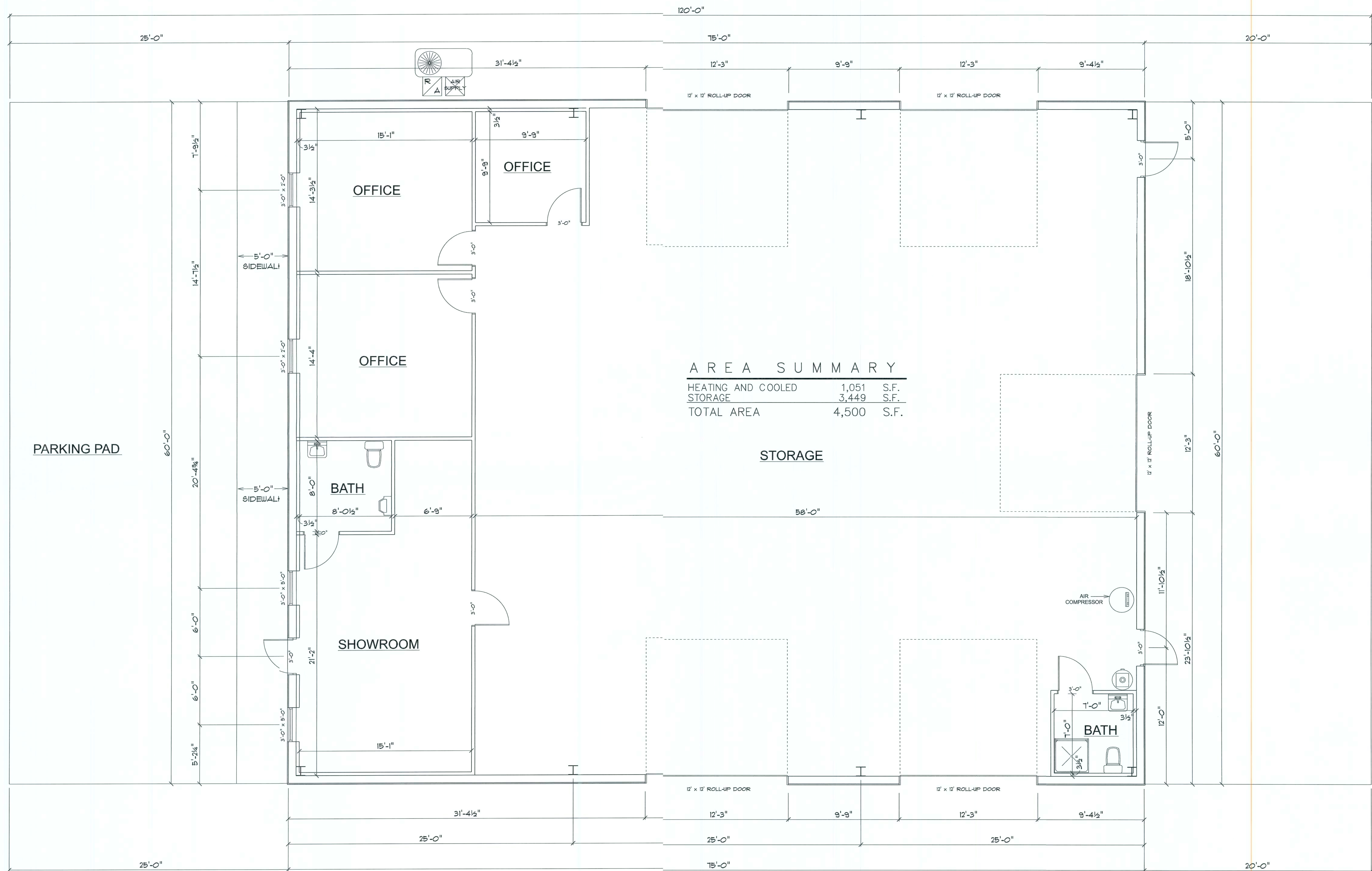
DIMENSIONED FLOOR PLAN SCALE: 1/4" = 1'-0"
