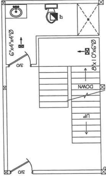
2nd FLR HVAC PLAN 1/8" = 1'-0"
