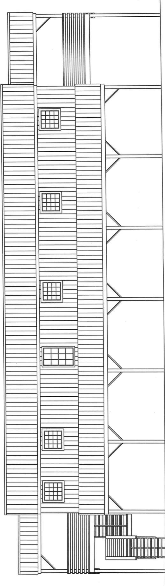
EAST ELEVATION 1/8" = 1'-0"
