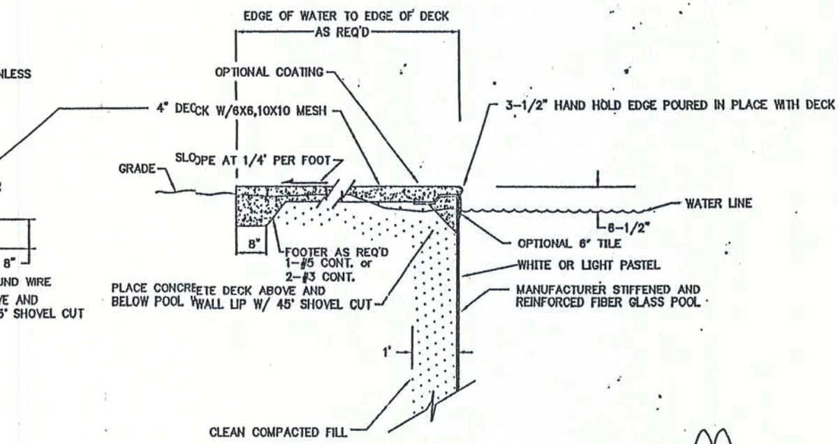
WALL SECTION NOT TO SCALE
