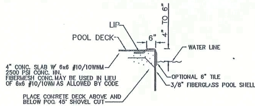
ALTERNATE COPING DETAIL NOT TO SCALE
