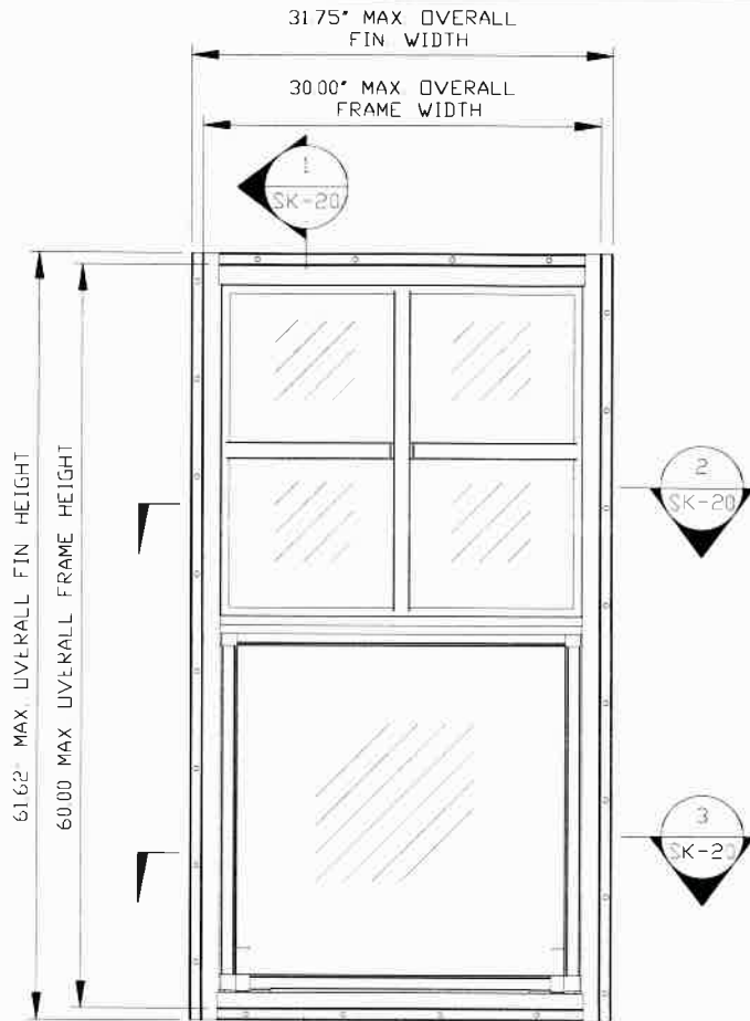
ELEVATION VIEW
