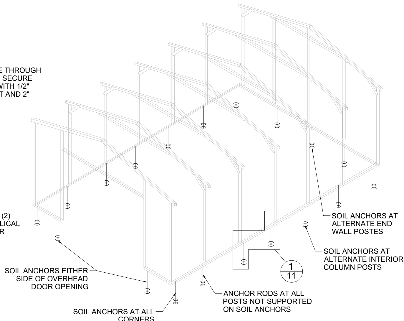
SOIL FOUNDATION
