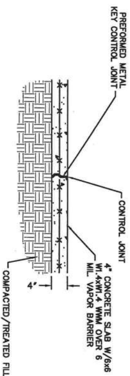
D-E DETAIL D (TYP.) S-2 CONTROL JOINT
