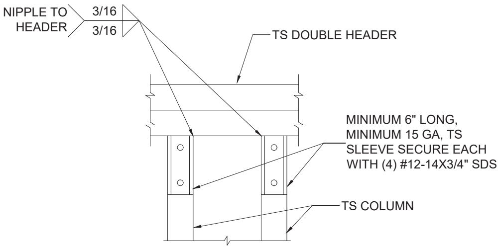
11 DOUBLE HEADER TO POST CONNECTION SCALE: NTS
