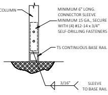
2 SIDEWALL SINGLE COLUMN/BASE RAIL CONNECTION DETAIL SCALE: NTS
