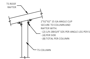
END COLUMN/RAFTER CONNECTION SCALE: NTS
