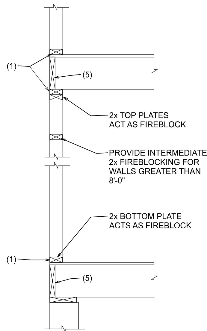
PLATFORM FRAMING
