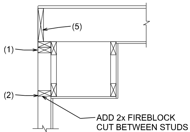
SOFFIT/DROPPED CLG.
