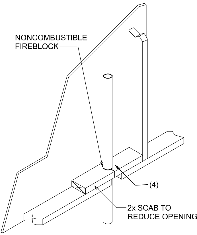
PENETRATIONS
