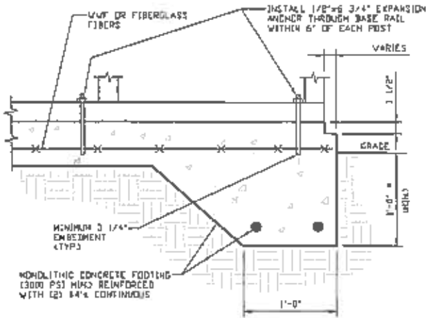
SCALE: NTS (MINIMUM ANCHOR EDGE DISTANCE IS 4") * COORDINATE WITH LOCAL CODES/ORD.
