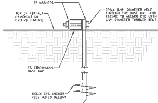
SCALE: NTS (CAN BE USED FOR ASPHALT)
