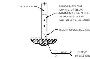
2 SIDEWALL SINGLE COLUMN/BASE RAIL CONNECTION DETAIL SCALE: NTS
