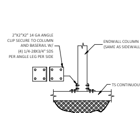
2C ENDWALL COLUMN/BASE RAIL CONNECTION DETAIL SCALE: NTS
