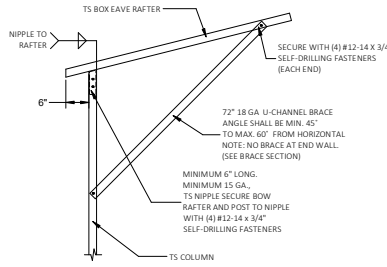
1 BOX EAVE RAFTER COLUMN CONNECTION DETAIL FOR HEIGHTS 13'-0" < TO <= 14'-0" SCALE: NTS
