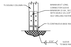
2A SIDEWALL DOUBLE COLUMN/BASE RAIL CONNECTION DETAIL SCALE: NTS
