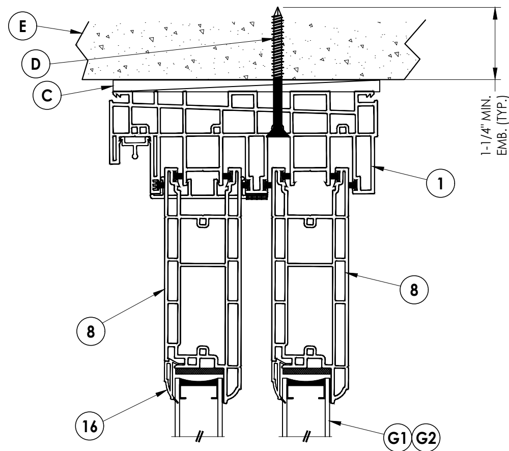
1 VERTICAL CROSS SECTION 3 Shown w/ Direct to Masonry option
