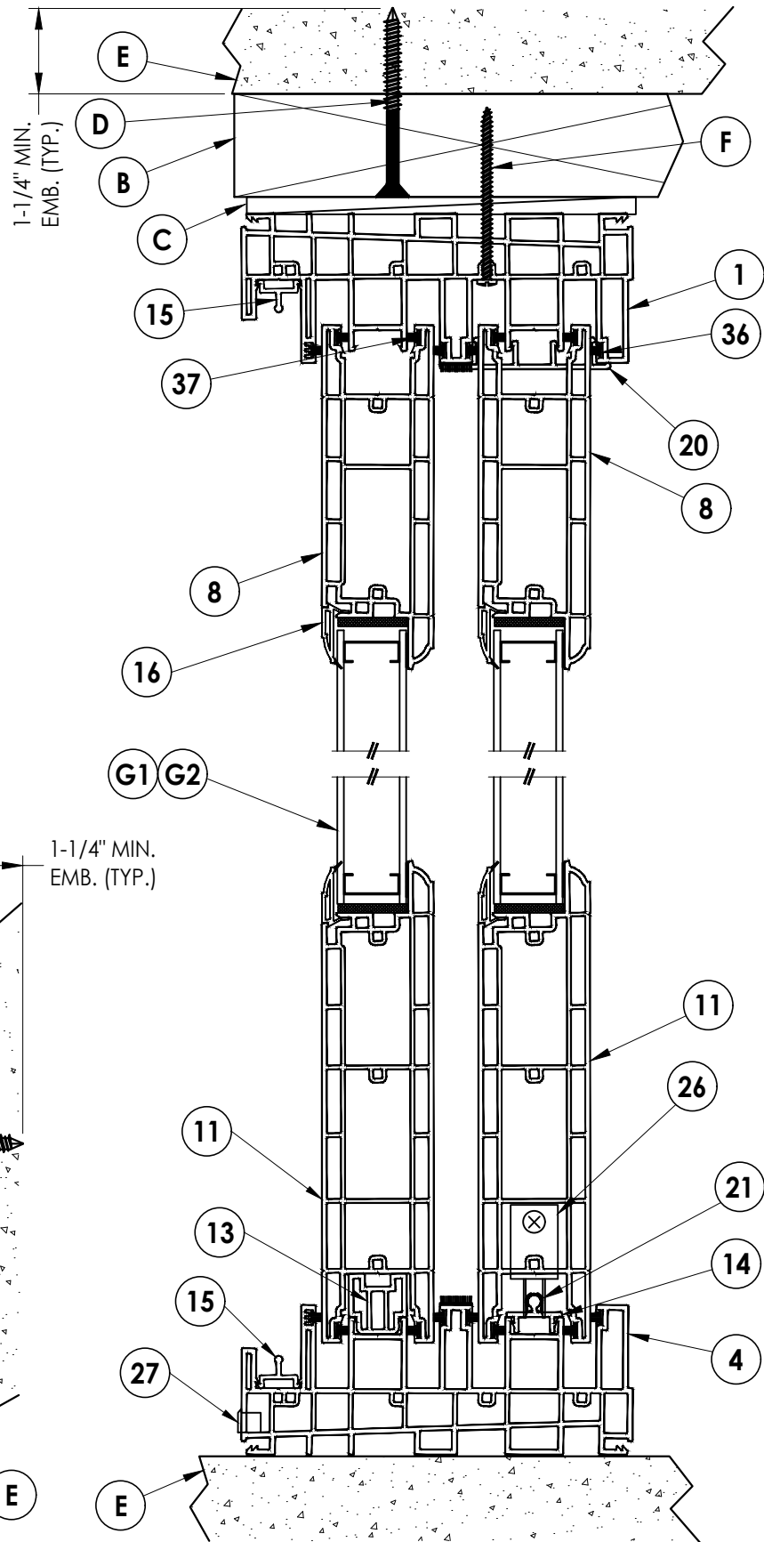
3 2 VERTICAL CROSS SECTION Shown w/ Direct to Masonry @ Sill
