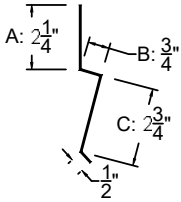
REGULAR STUCCO (6")
