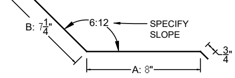
TRANSITION (16")
