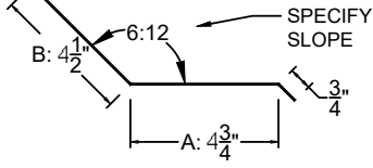
HEADWALL (10")
