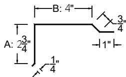
GABLE (8.75")
