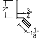
FIRST STUCCO (6")
