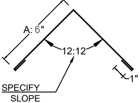
FLAT CAP (14")
