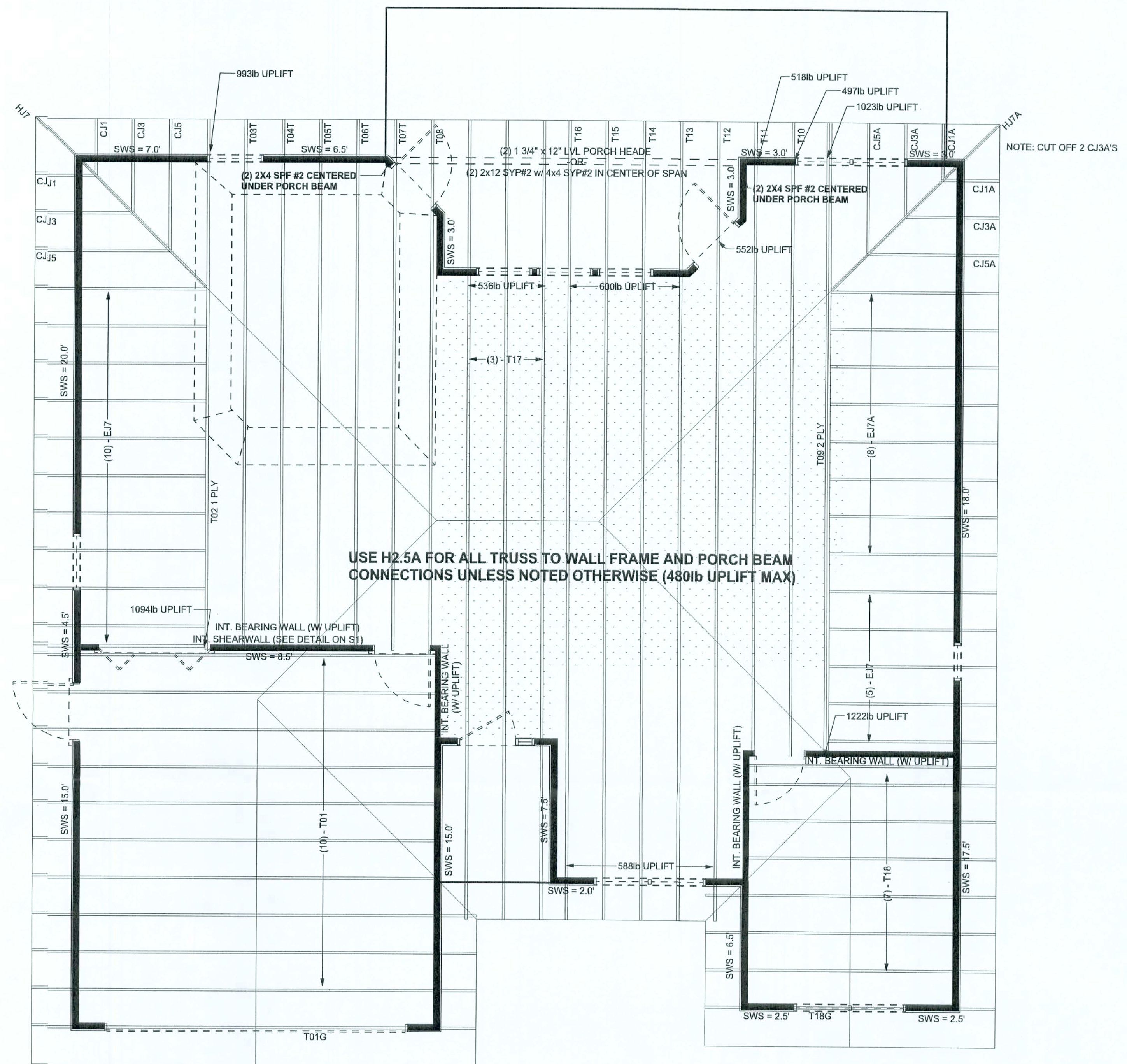
STRUCTURAL LAYOUT
