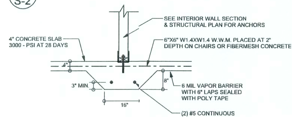
F2 INTERIOR BEARING FOOTING
