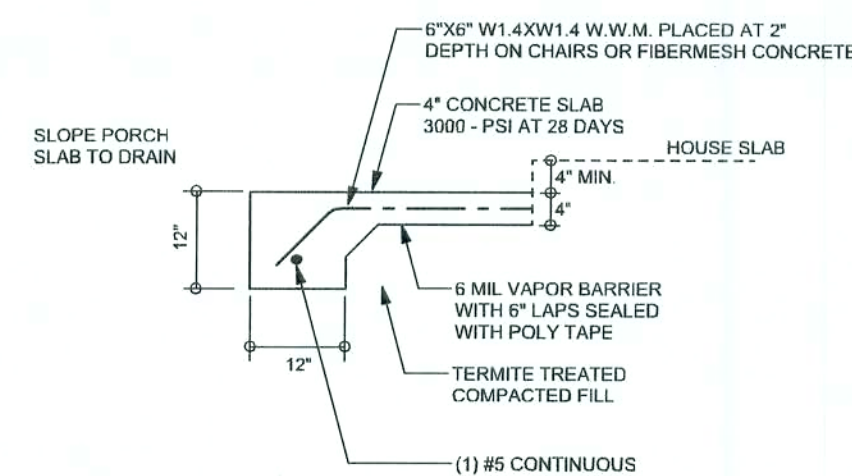
F5 PORCH FOOTING
