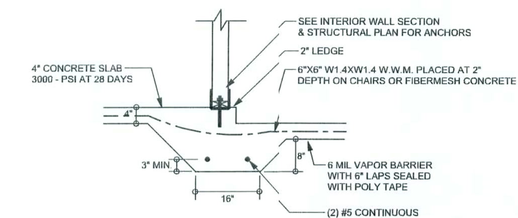
F3 INTERIOR BEARING STEP FOOTING WITH 2" LEDGE
