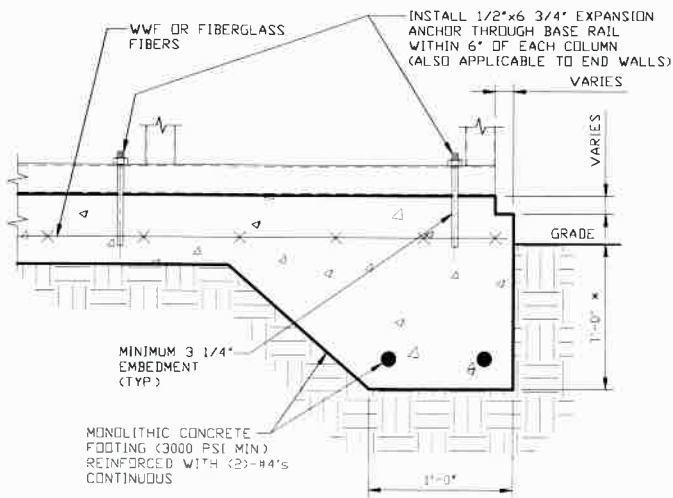
CONCRETE MONOLITHIC SLAB BASE RAIL ANCHORAGE
