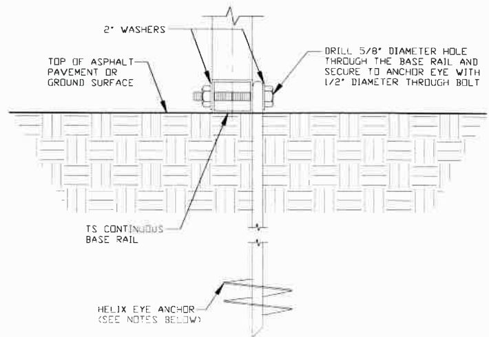
GROUND BASE HELIX ANCHORAGE
