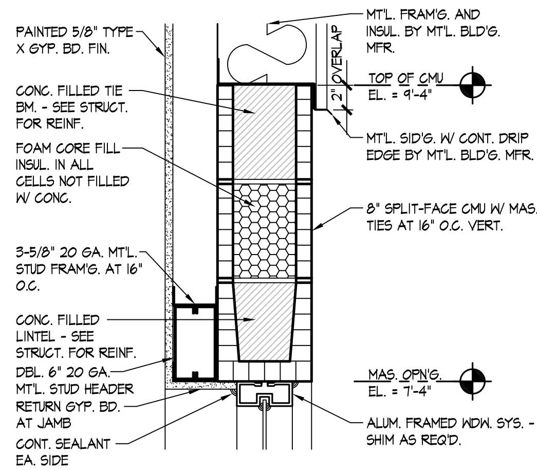
WINDOW HEAD DETAIL 1-1/2" = 1'-0"
