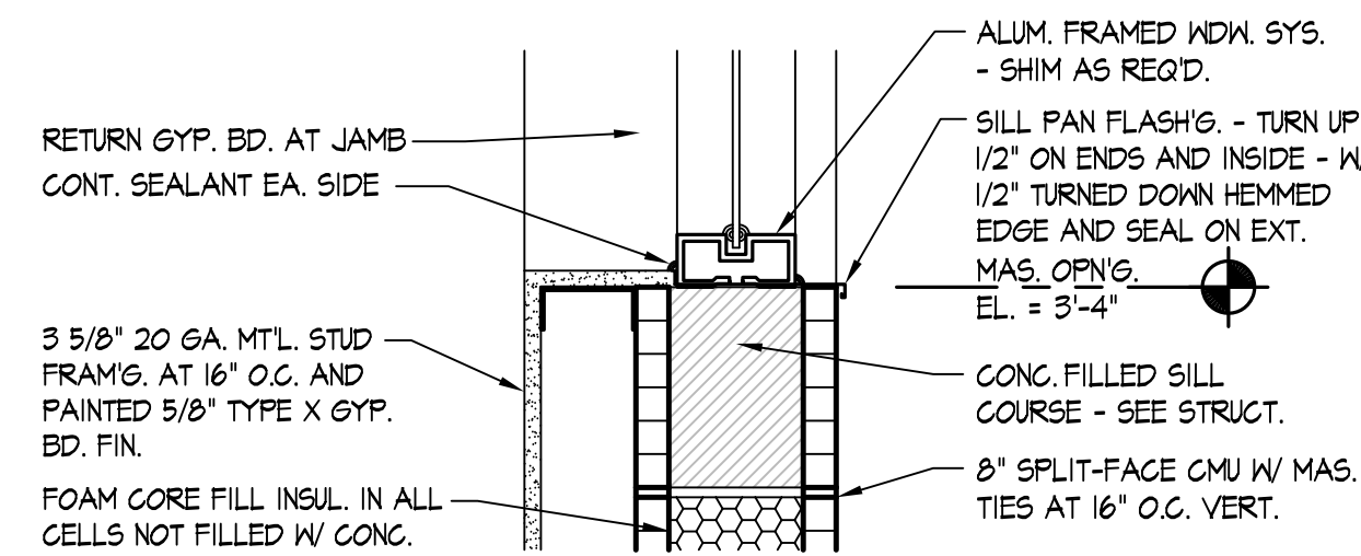
WINDOW SILL DETAIL 1-1/2" = 1'-0"
