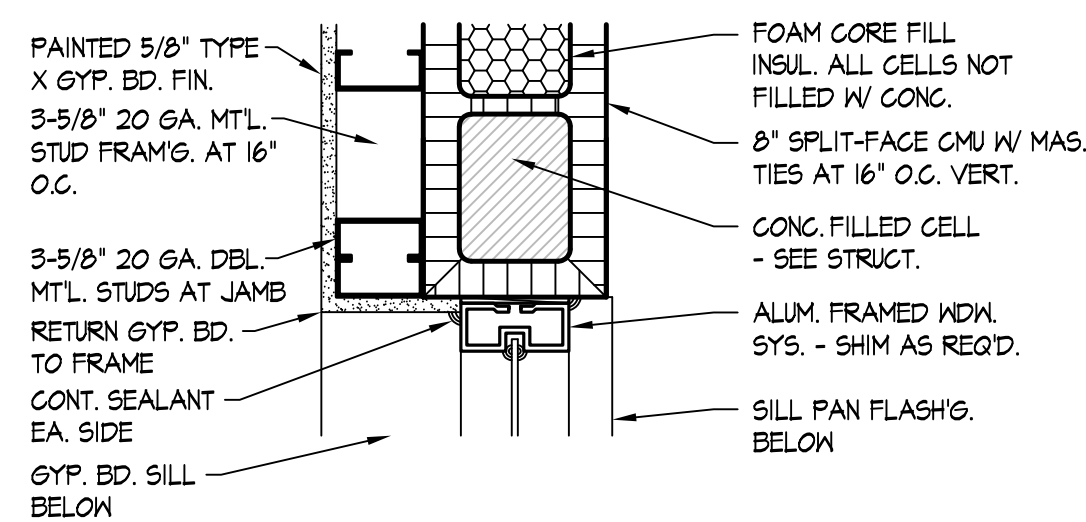
WINDOW JAMB DETAIL 1-1/2" = 1'-0"
