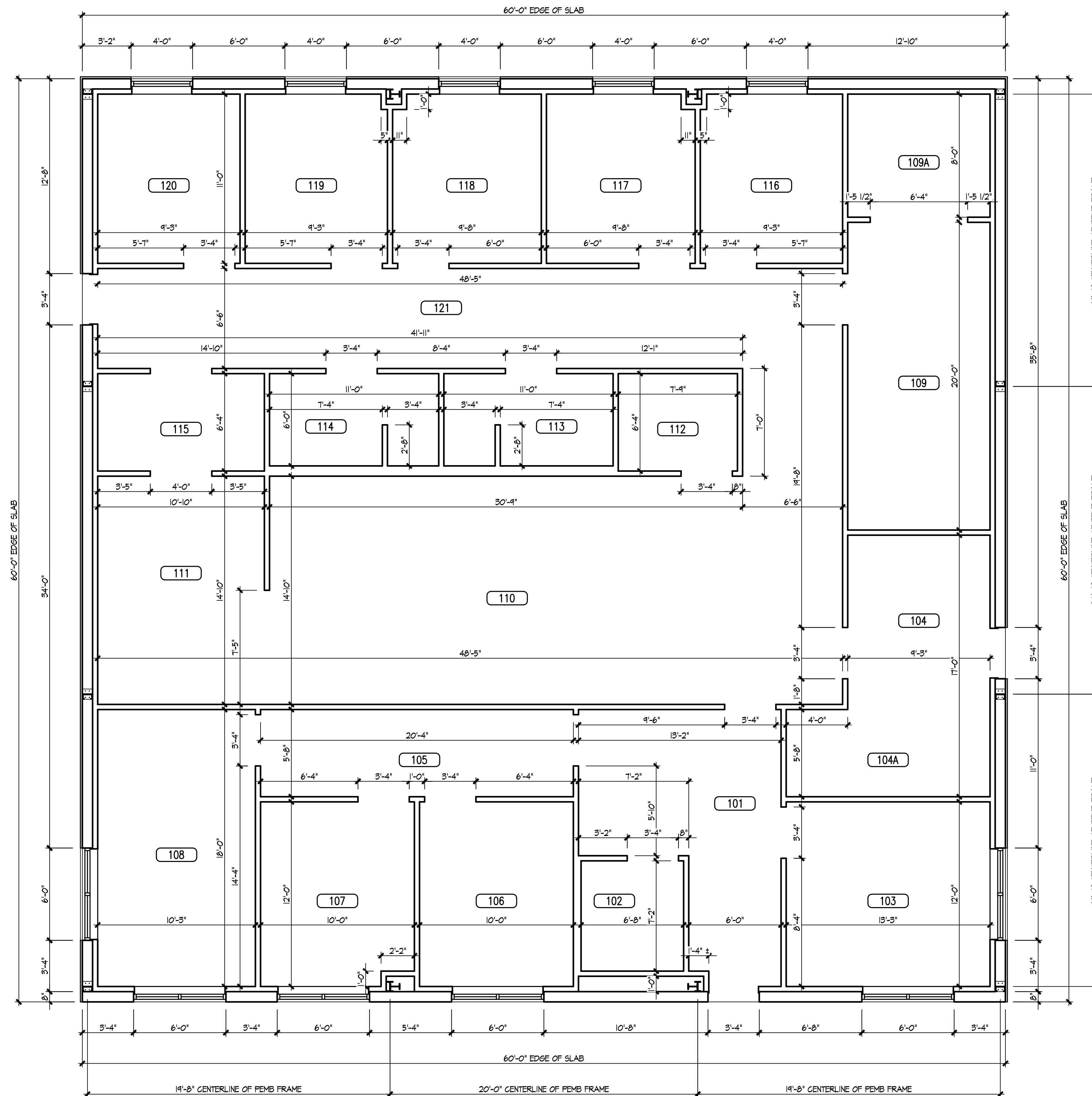
DIMENSION PLAN 1/4" = 1'-0"
