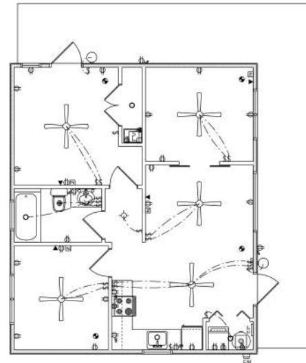
ELECTRICAL FLOOR PLAN SCALE: 1/8" = 1'-0"
