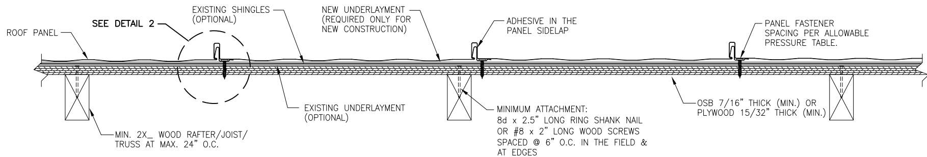
FASTENING PATTERN 2
