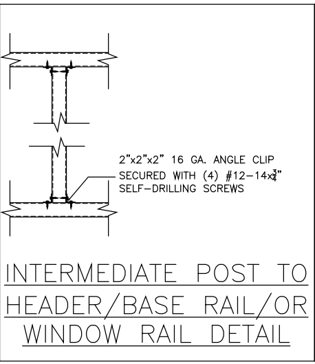
INTERMEDIATE POST TO HEADER/BASE RAIL/OR WINDOW RAIL DETAIL
