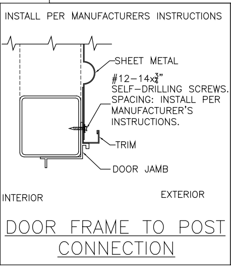
DOOR FRAME TO POST CONNECTION
