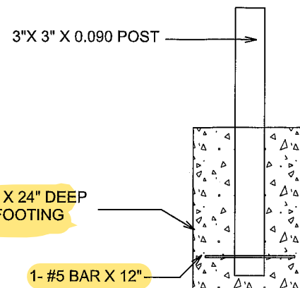
POST FOOTING 3\"/>
