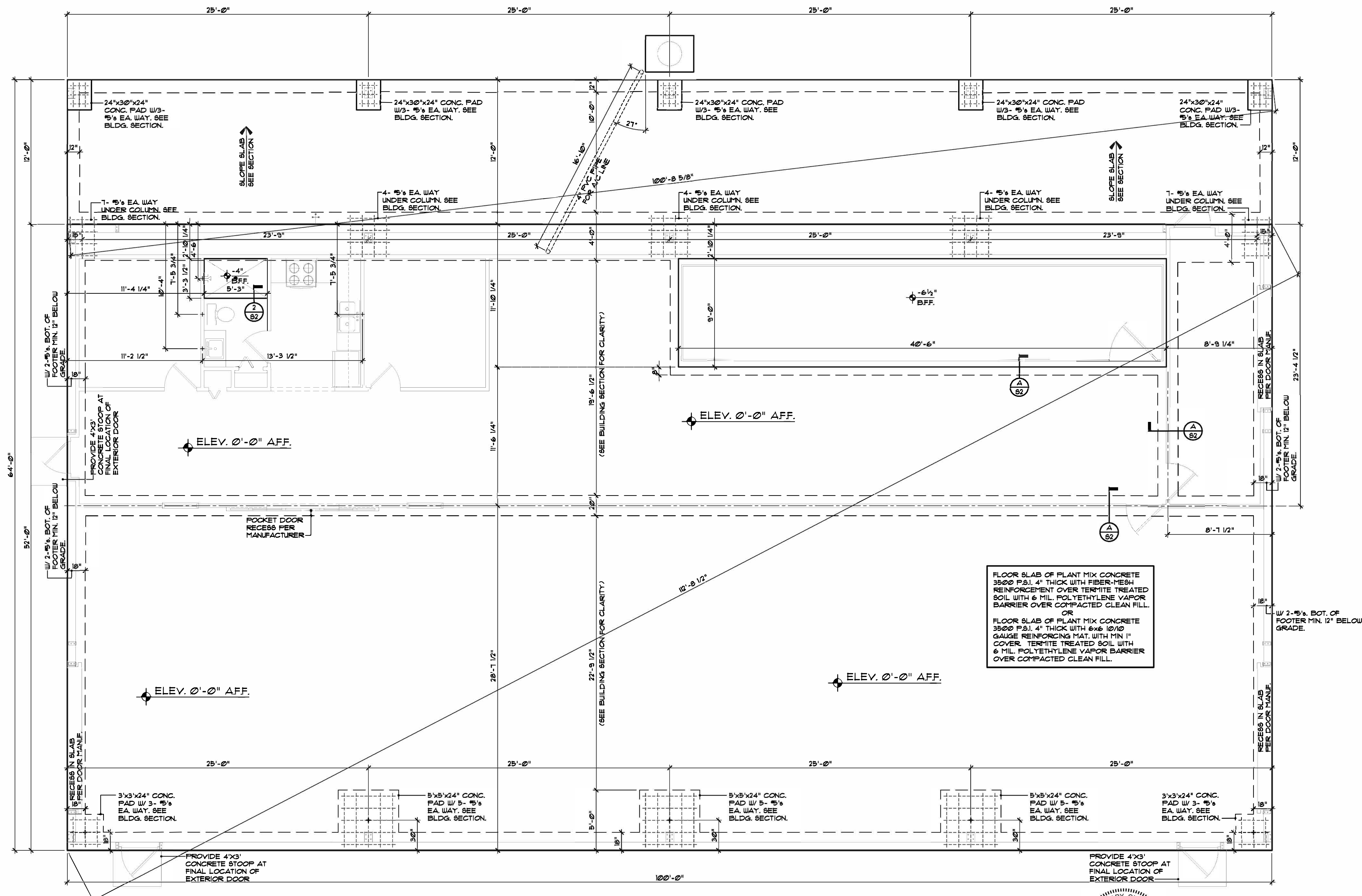
Foundation Plan SCALE: 1/4" = 1'-0" SEE BUILDING SECTION FOR PERIMETER FOOTERS
