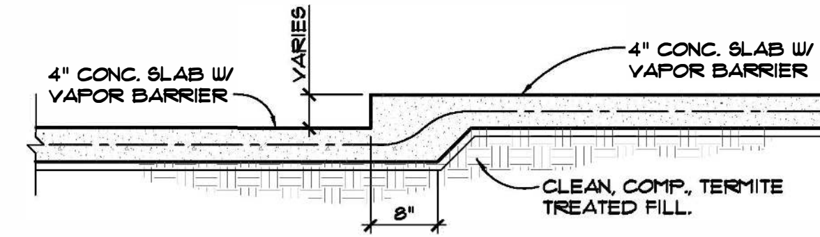
2 Step in Slab, Non Bearing SCALE: 3/4" = 1'-0"
