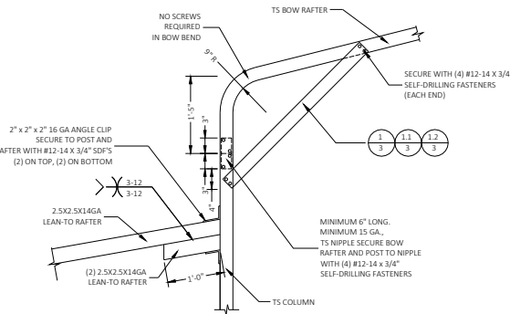
SIDE EXTENSION RAFTER/COLUMN DETAIL FOR EXTENSION RAFTER SPANS 12'-0" < W \leq 16'-0" , IF THE KNEE BRACE ON THE OTHER END OF THE RAFTER IS PER DETAIL 1.2/3. FOR EXTENSION RAFTER SPANS 13'-0" < W \leq 18'-0" , IF THE KNEE BRACE ON THE OTHER END OF THE RAFTER IS PER DETAIL 1.1/3. FOR EXTENSION RAFTER SPANS 15'-0" < W \leq 19'-0" , IF THE KNEE BRACE ON THE OTHER END OF THE RAFTER IS PER DETAIL 1/3. SCALE: NTS
