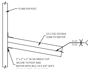
LEAN-TO RAFTER TO RAFTER COLUMN CONNECTION DETAIL FOR LEAN-TO RAFTER SPANS 16'-0" < W \leq 24'-0" , IF THE KNEE BRACE ON THE OTHER END OF THE RAFTER IS PER DETAIL 1.2/2 OR 1.2/3. FOR LEAN-TO RAFTER SPANS 18'-0" < W \leq 24'-0" , IF THE KNEE BRACE ON THE OTHER END OF THE RAFTER IS PER DETAIL 1.1/2 OR 1.1/3. FOR LEAN-TO RAFTER SPANS 19'-0" < W \leq 24'-0" , IF THE KNEE BRACE ON THE OTHER END OF THE RAFTER IS PER DETAIL 1/2 OR 1/3. SCALE: NTS
