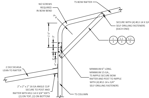
SIDE EXTENSION RAFTER/COLUMN DETAIL FOR EXTENSION RAFTER SPANS W \leq 12'-0" , IF THE KNEE BRACE ON THE OTHER END OF THE RAFTER IS PER DETAIL 1.2/3. FOR EXTENSION RAFTER SPANS W \leq 13'-0" , IF THE KNEE BRACE ON THE OTHER END OF THE RAFTER IS PER DETAIL 1.1/3. FOR EXTENSION RAFTER SPANS W \leq 15'-0" , IF THE KNEE BRACE ON THE OTHER END OF THE RAFTER IS PER DETAIL 1/3. SCALE: NTS
