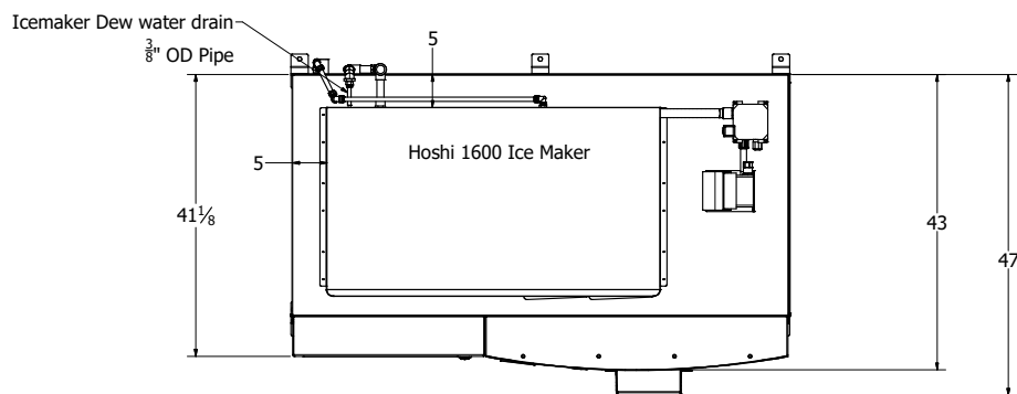
VIEW L-L SCALE 1:10
