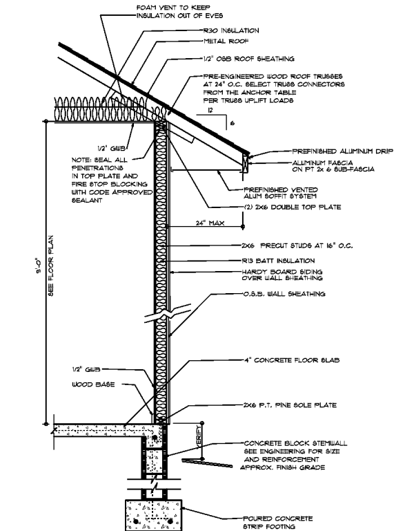
TYPICAL DESIGN WALL SECTION NON - STRUCTURAL DATA
