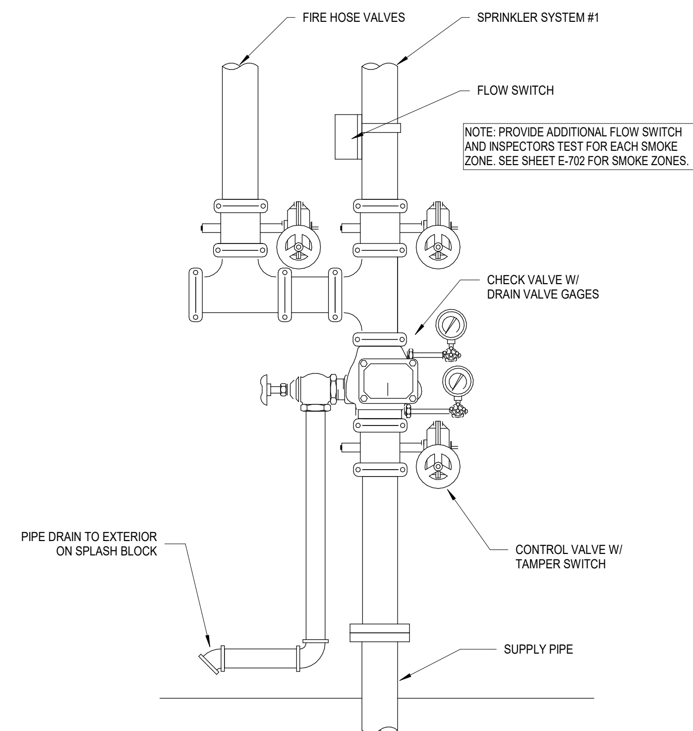
SPRINKLER RISER - WET PIPE SYSTEM
