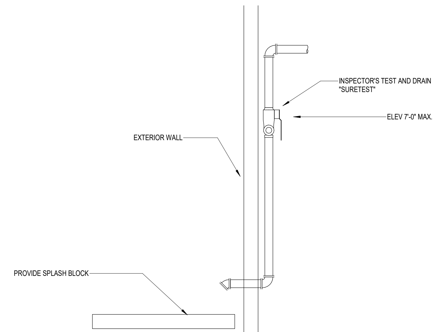
INSPECTOR'S TEST - WET PIPE SYSTEM
