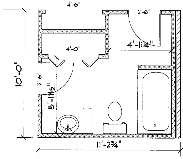
New Bath Layout
