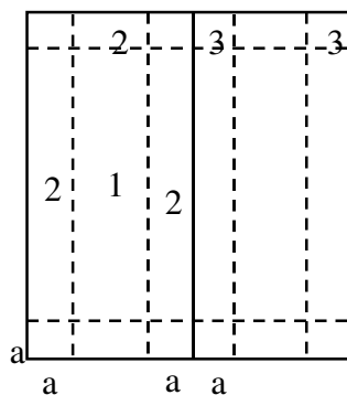
Figure 6-5 - External Pressure Coefficients, GCp Loads on Components and Cladding for Buildings w/ Ht ≤ 60 ft
