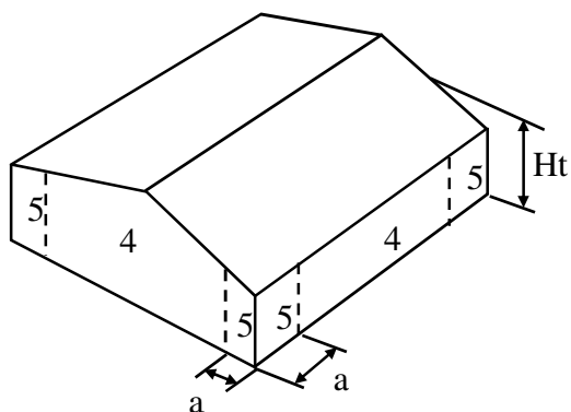
Figure 6-5 - External Pressure Coefficients, GCp Loads on Components and Cladding for Buildings w/ Ht ≤ 60 ft
