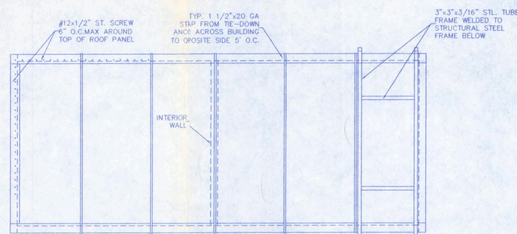
ROOF PLAN
