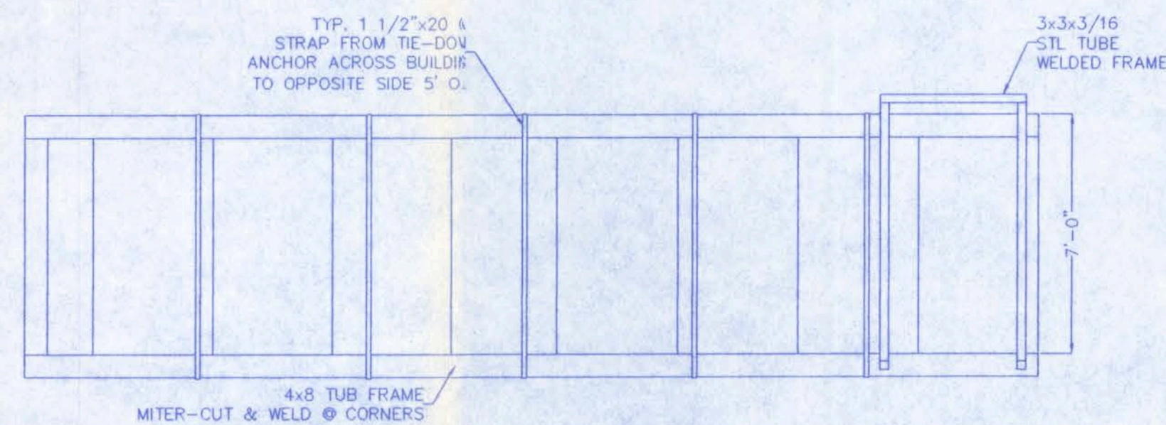
SIDE ELEV. VIEW
