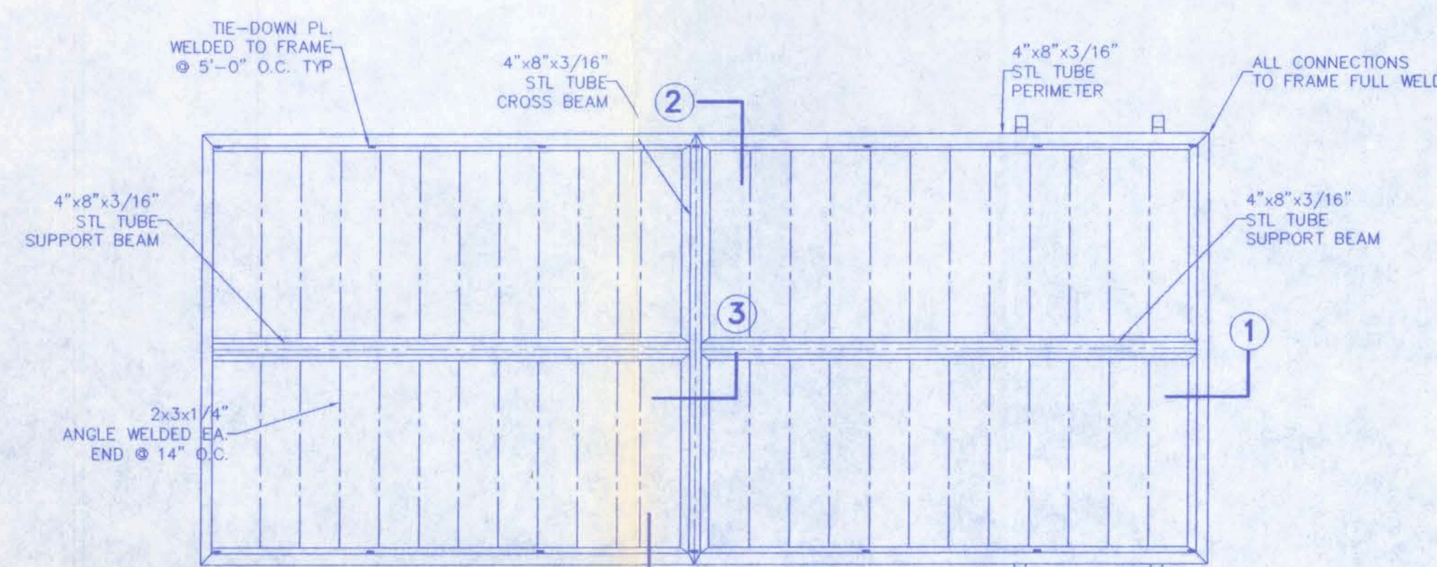
FRAME PLAN
