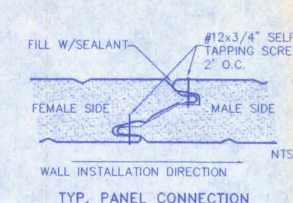
TYP. PANEL CONNECTION
