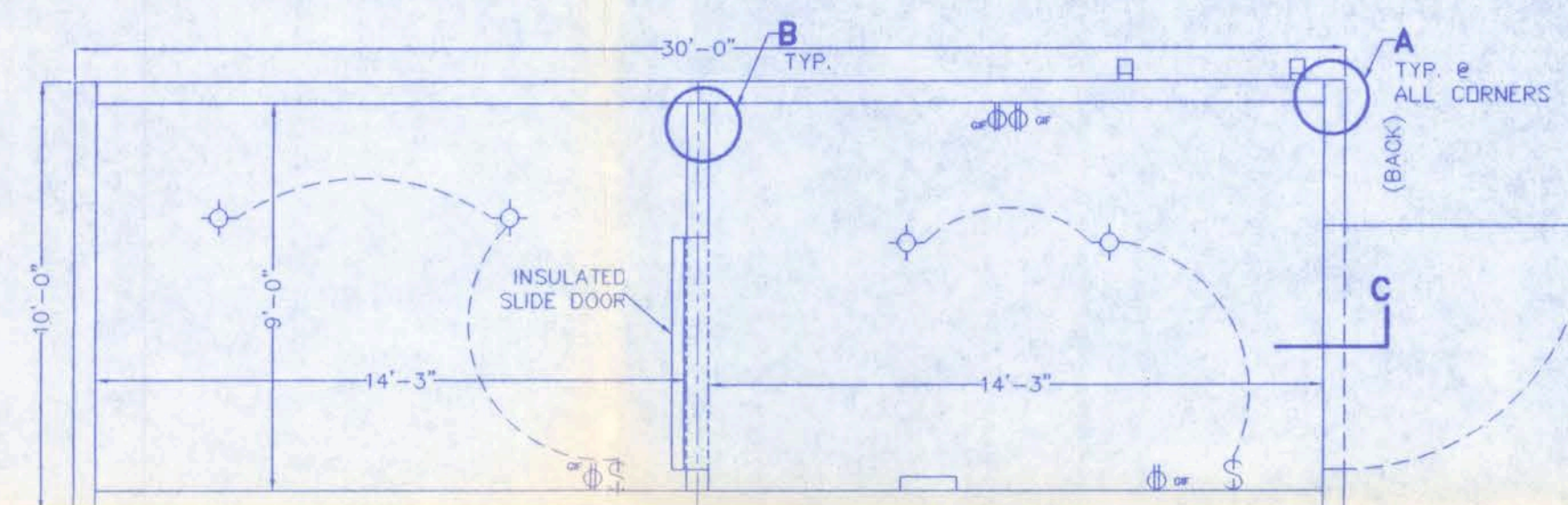
FLOOR PLAN
