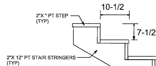
STAIR DETAIL
