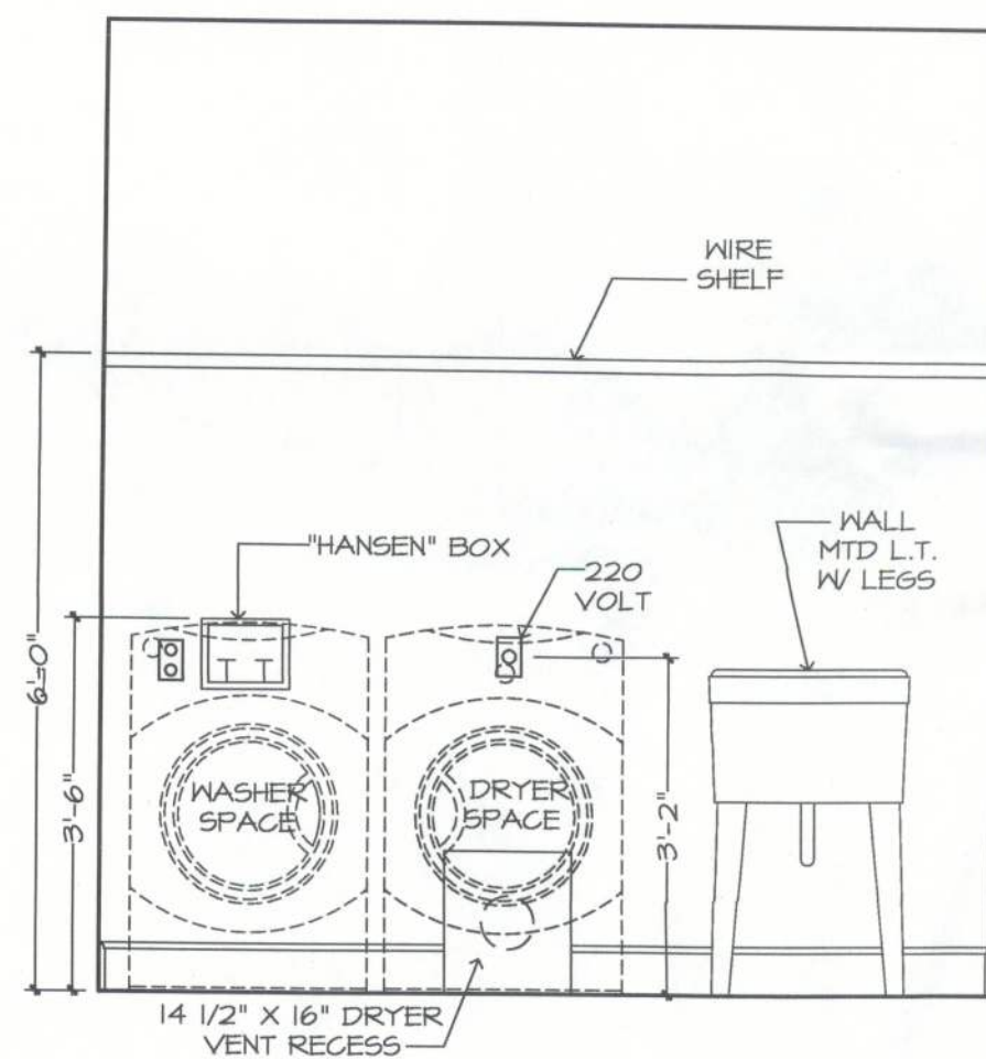
WALL "W" UTILITY
