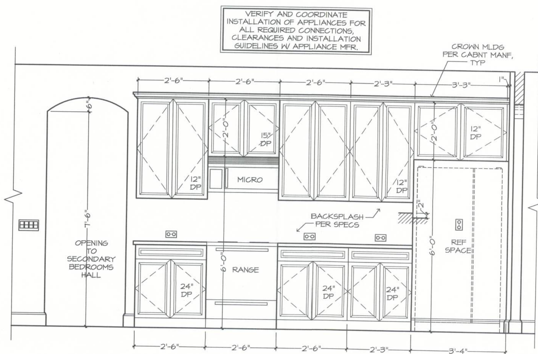
WALL "Y" KITCHEN
