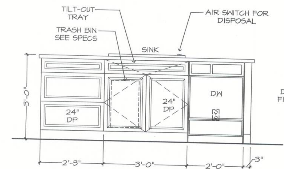
FRONT VIEW KITCHEN ISLAND
