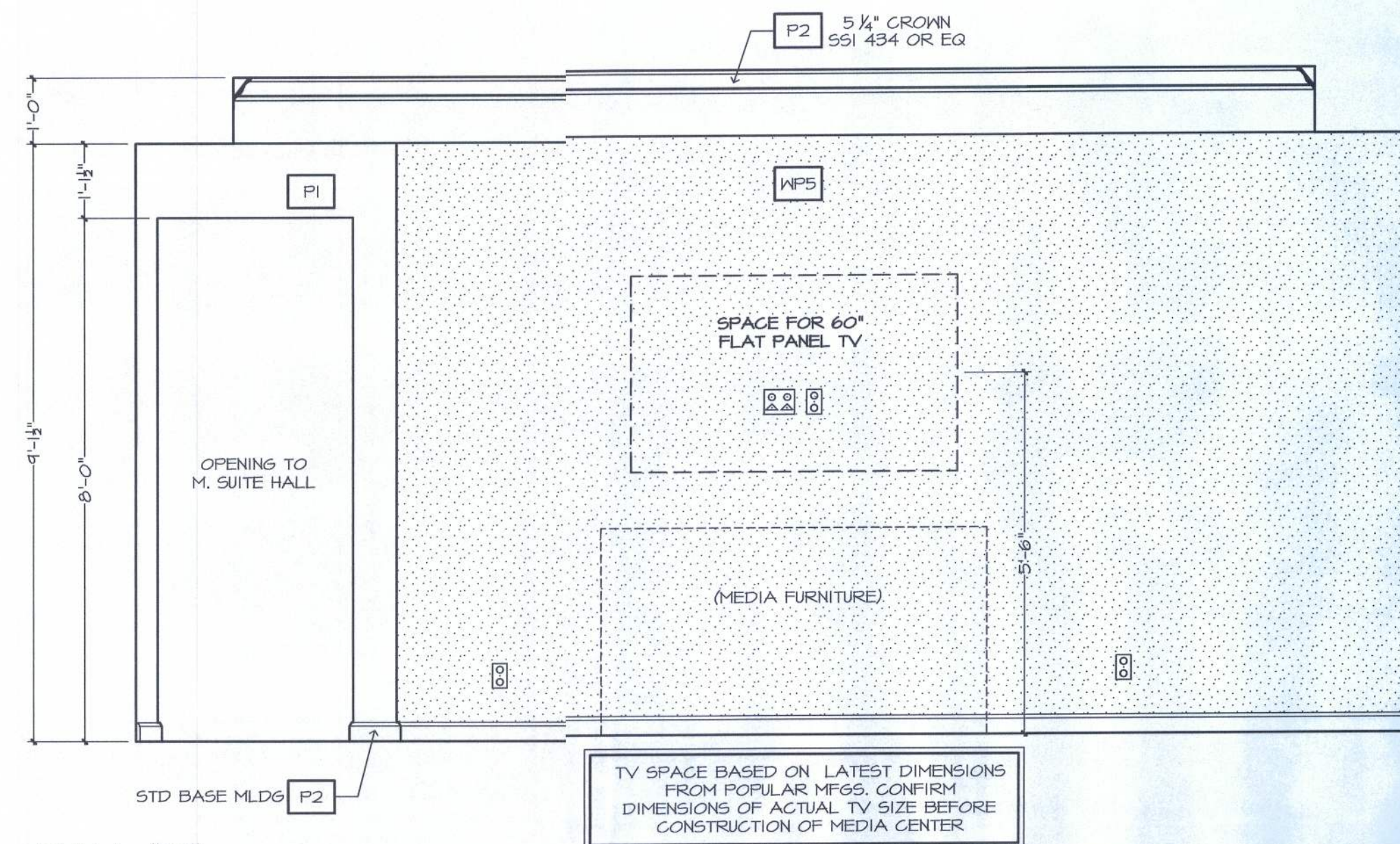
WALL "W" GREAT ROOM
