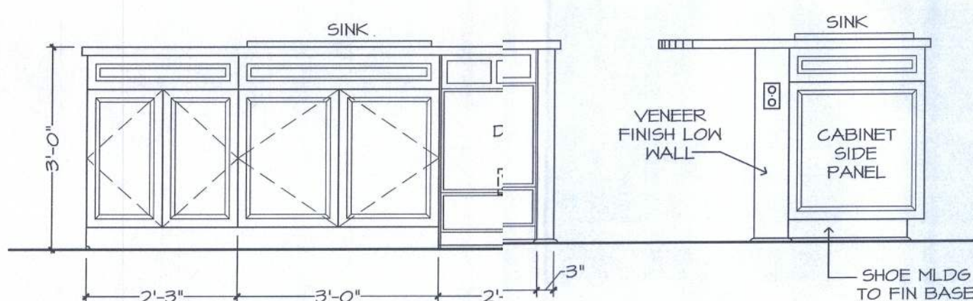
FRONT VIEW KITCHEN ISLAND
