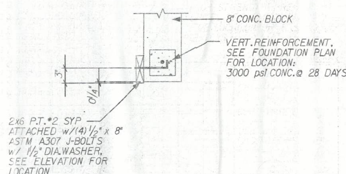
GARAGE DOOR BUCK DETAIL
