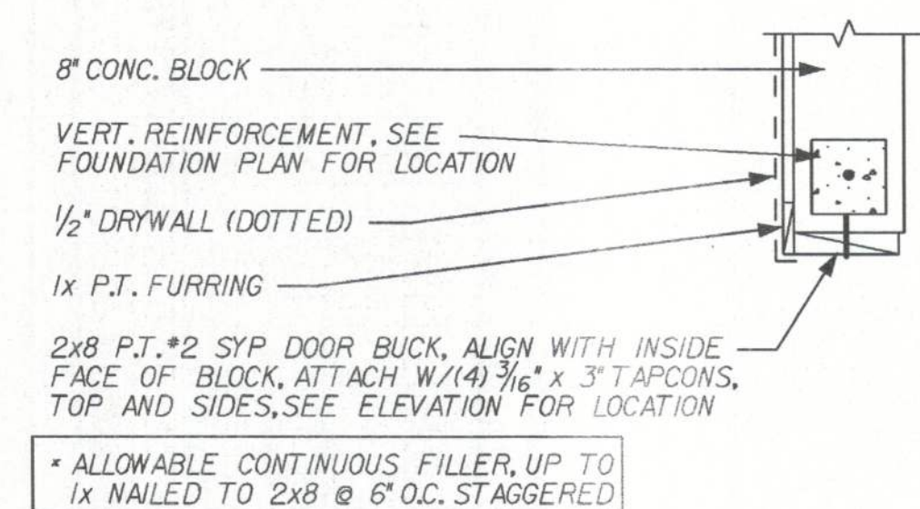
SLIDING GLASS DOOR BUCK DETAIL
