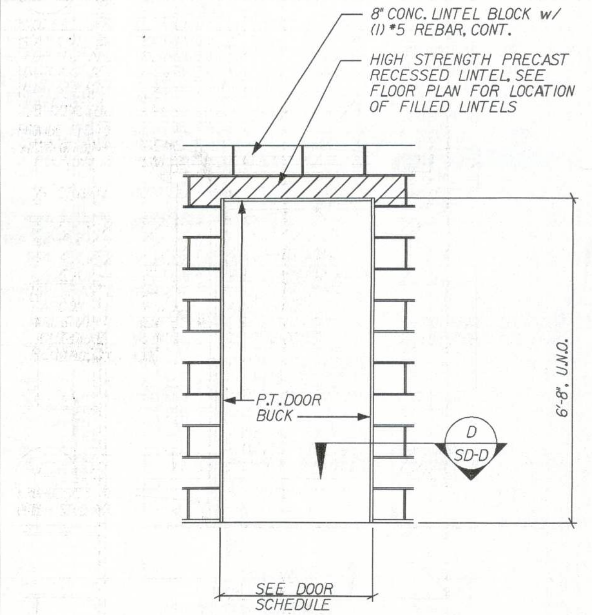
STANDARD DOOR ELEVATION
