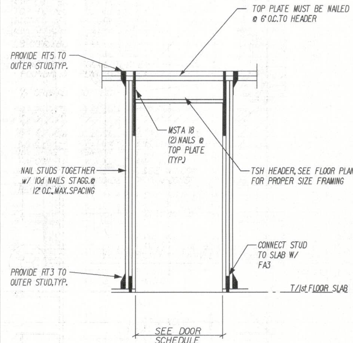
FRM'G @ SHEAR WALL : UPLIFT
