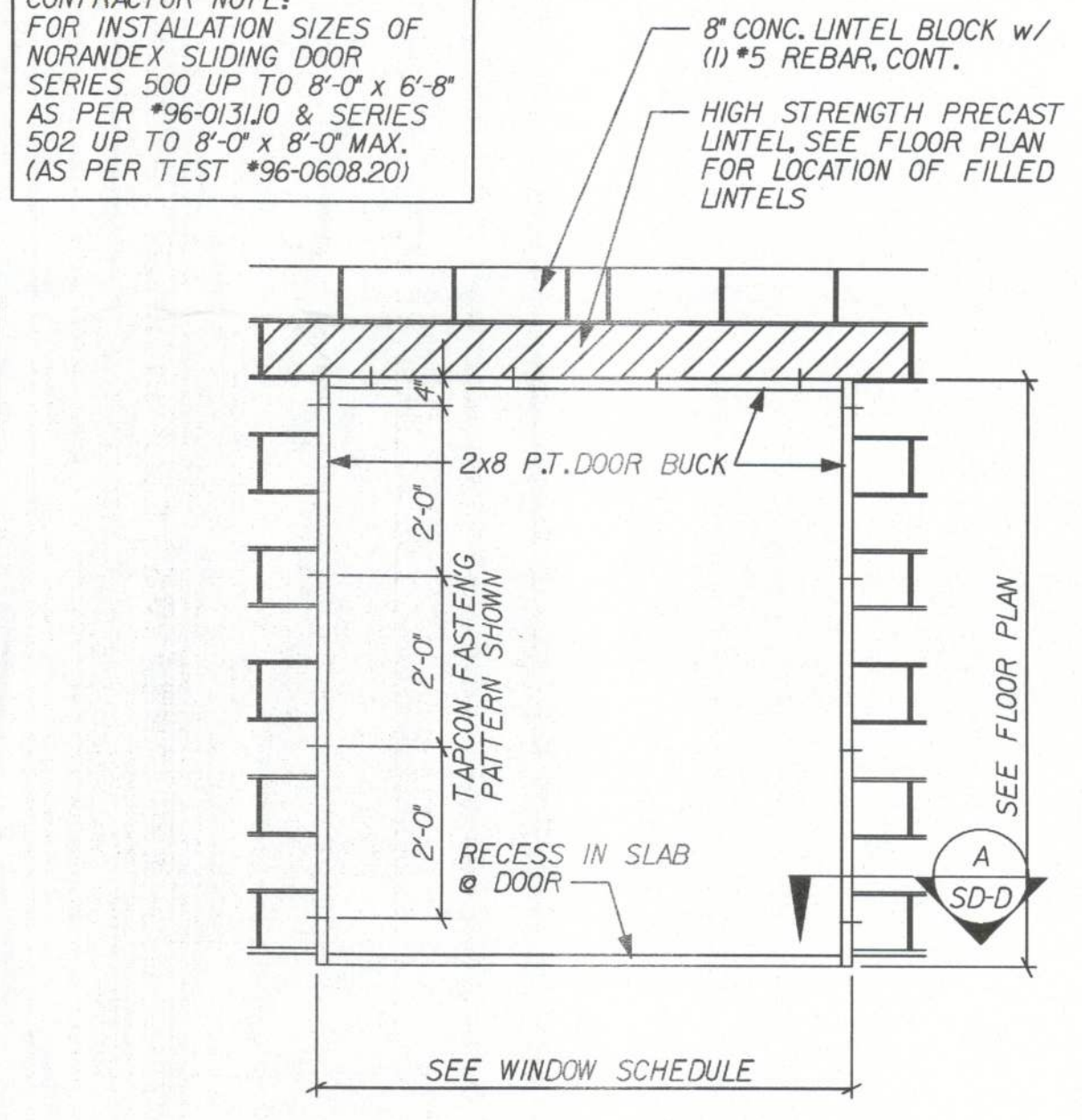
SLIDING GLASS DOOR ELEVATION
