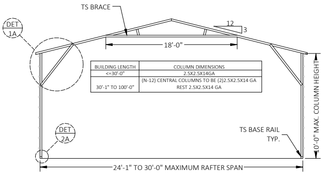
TRUSS LAYOUT- BOX EAVE
