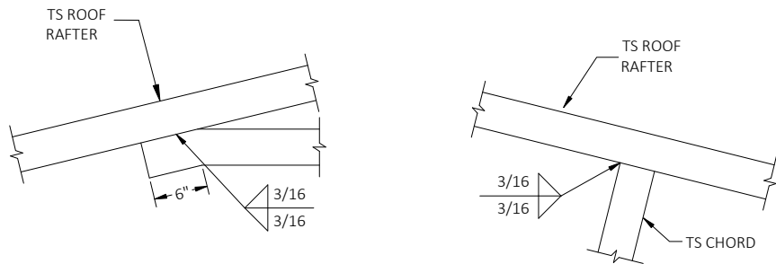
DETAIL 9 COLLAR TIE CONNECTION
