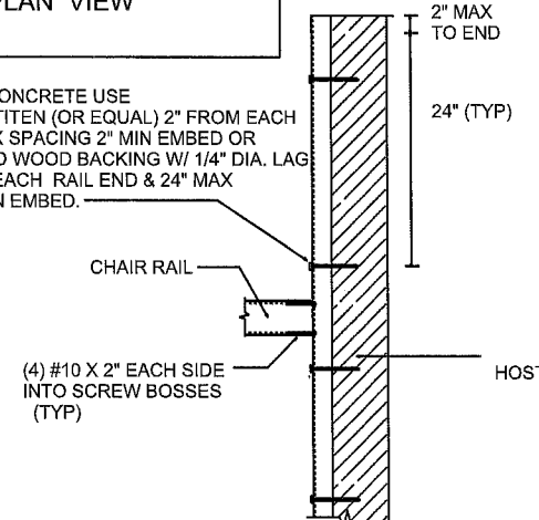
RAIL TO HOST @ CHAIR RAIL CONNECTION WOOD OR MASONRY HOST CHOOSE CONNECTOR THAT IS APPLICABLE N.T.S.
