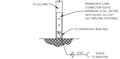
2 RAFTER POST/BASE RAIL CONNECTION DETAIL SCALE: NTS
