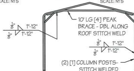
TYP. OPEN END WALL ON 3 SIDED ENCLOSED BUILDING SCALE: NTS
