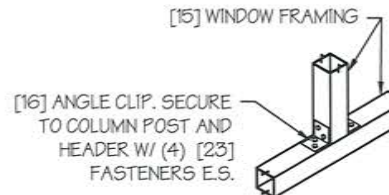
TYP. WINDOW FRAMING CONN. DETAIL 2 SCALE: NTS
