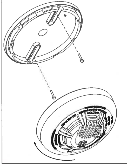
Fig 3. Mounting the detector
