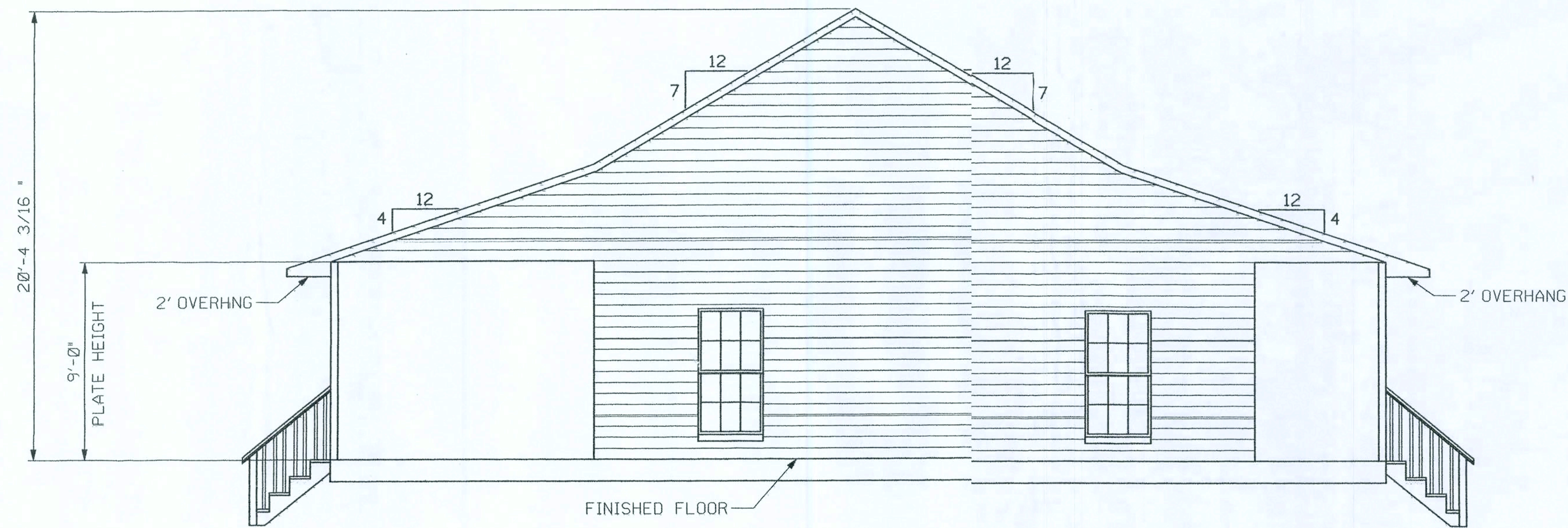
LEFT ELEVATION
