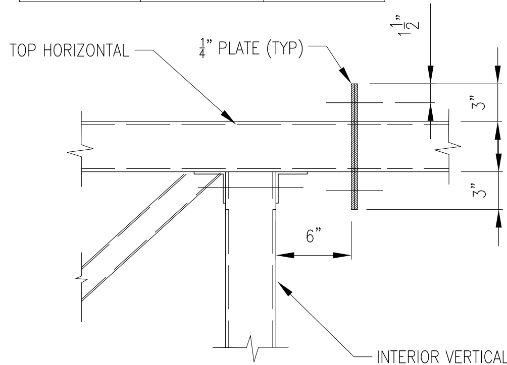
J TOP HORIZONTAL SPLICE - WITH SAG TRUSS REQUIRED FOR DOOR WIDTH >53' Scale: N.T.S.
