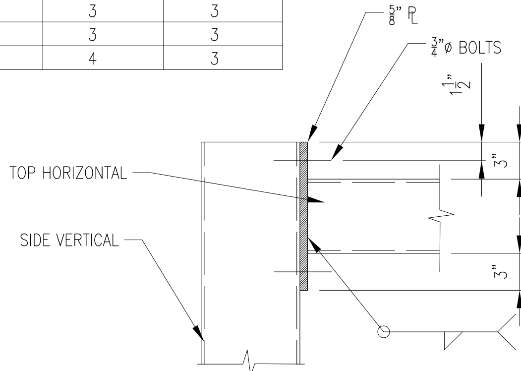
B TOP HORIZONTAL - SIDE VERTICAL (WITH SAG TRUSS) Scale: N.T.S.
