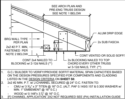
SF01 STRUCTURAL SOFFIT SCALE: 3/4" = 1'-0" @ 22x34 (**) SCALE: 3/8" = 1'-0" @ 11x17 REV. 03.26.2021 NOT REQUIRED. VINYL SOFFITS >1'-0" SHALL HAVE MID BLOCKING PER R704.2.1 REV. 09.10.2021 *REFER TO THE PRODUCT APPROVAL FOR INSTALLATION DETAILS.*
