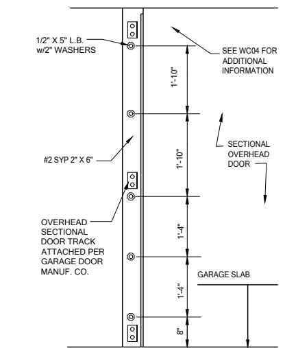
WC05 SECT. OVERHEAD GAR. DOOR INSTALL SCALE: 3/4" = 1'-0" @ 22x34 SCALE: 3/8" = 1'-0" @ 11x17
