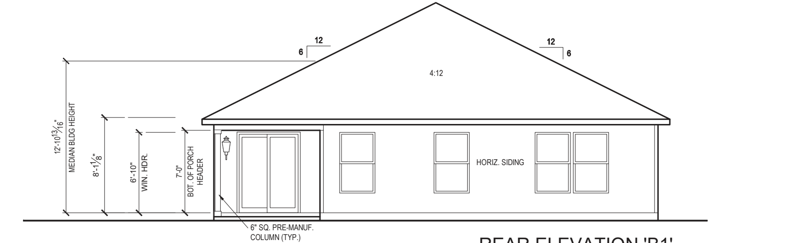
REAR ELEVATION 'B1'
