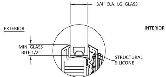
GLAZING DETAIL 1
