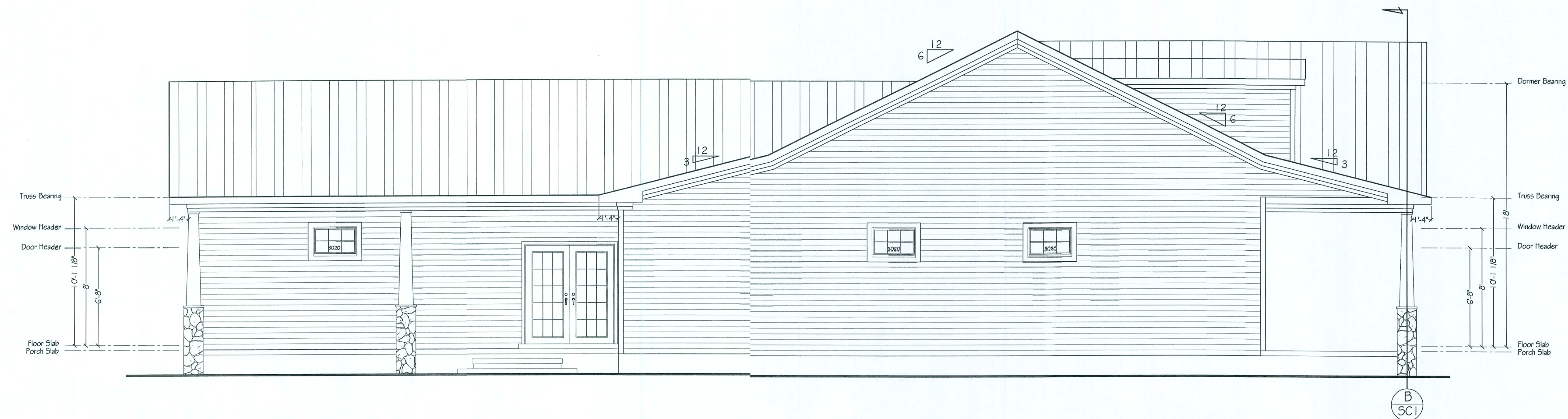
Left Elevation
