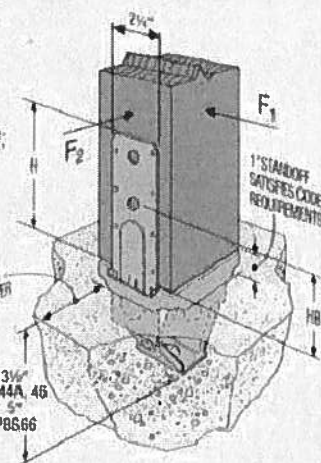
Typical PBS44A Installation
