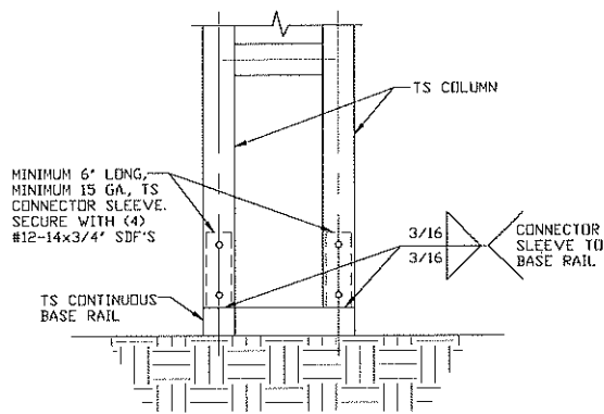
RAFTER COLUMN/BASE RAIL CONNECTION DETAIL SCALE: NTS
