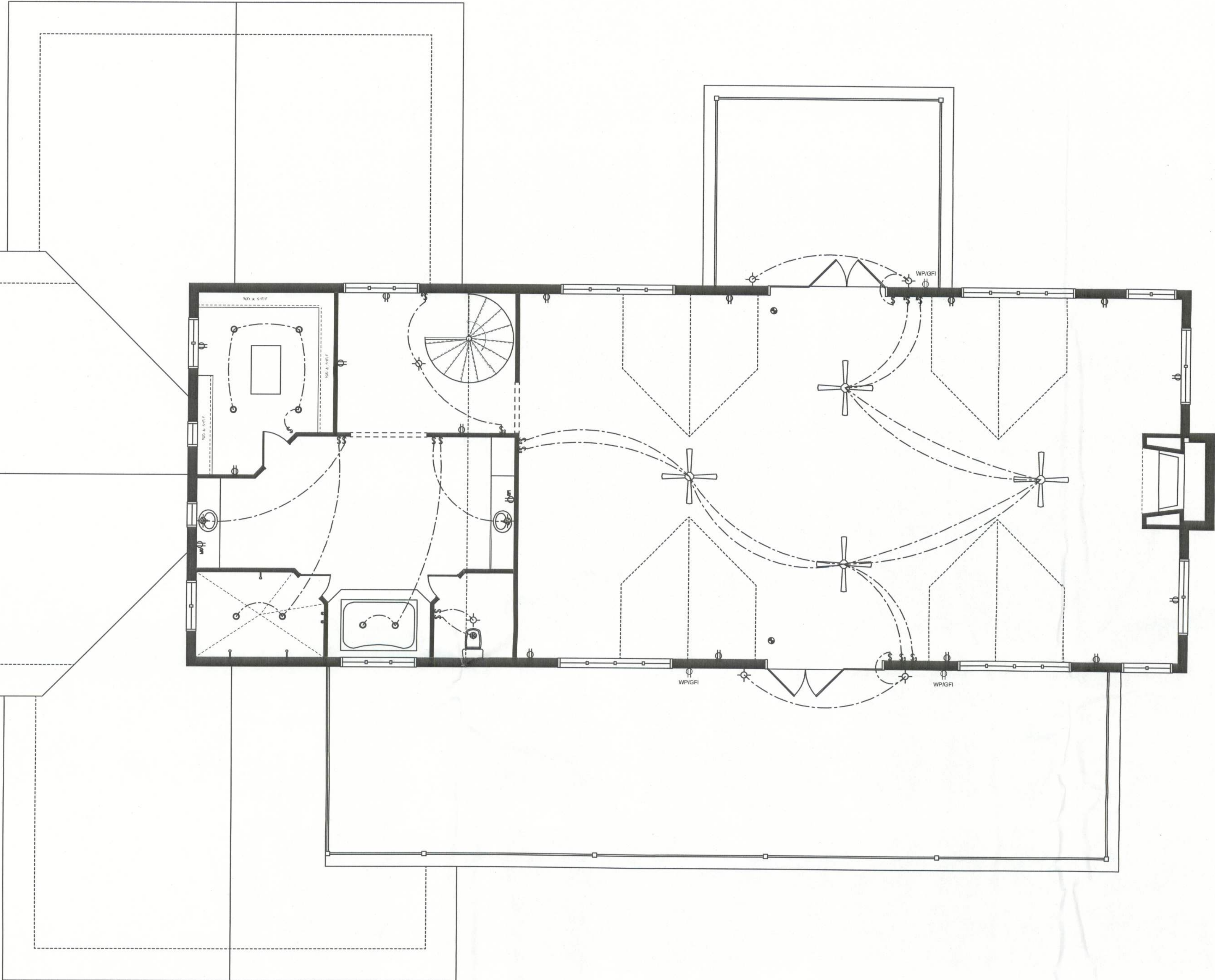
ELECTRICAL PLAN SCALE: 3/16" = 1'-0" NOTE: VERIFY ALL EXISTING ELECTRICAL!
