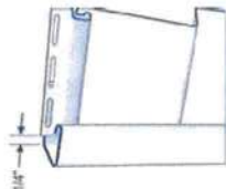
J-channel detail
