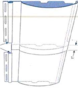
Adirondack panel junction detail
