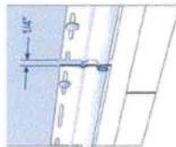
Starter trim installation weather-resistant barrier
