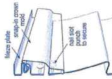
Top panel installation using frieze plate and crown mold
