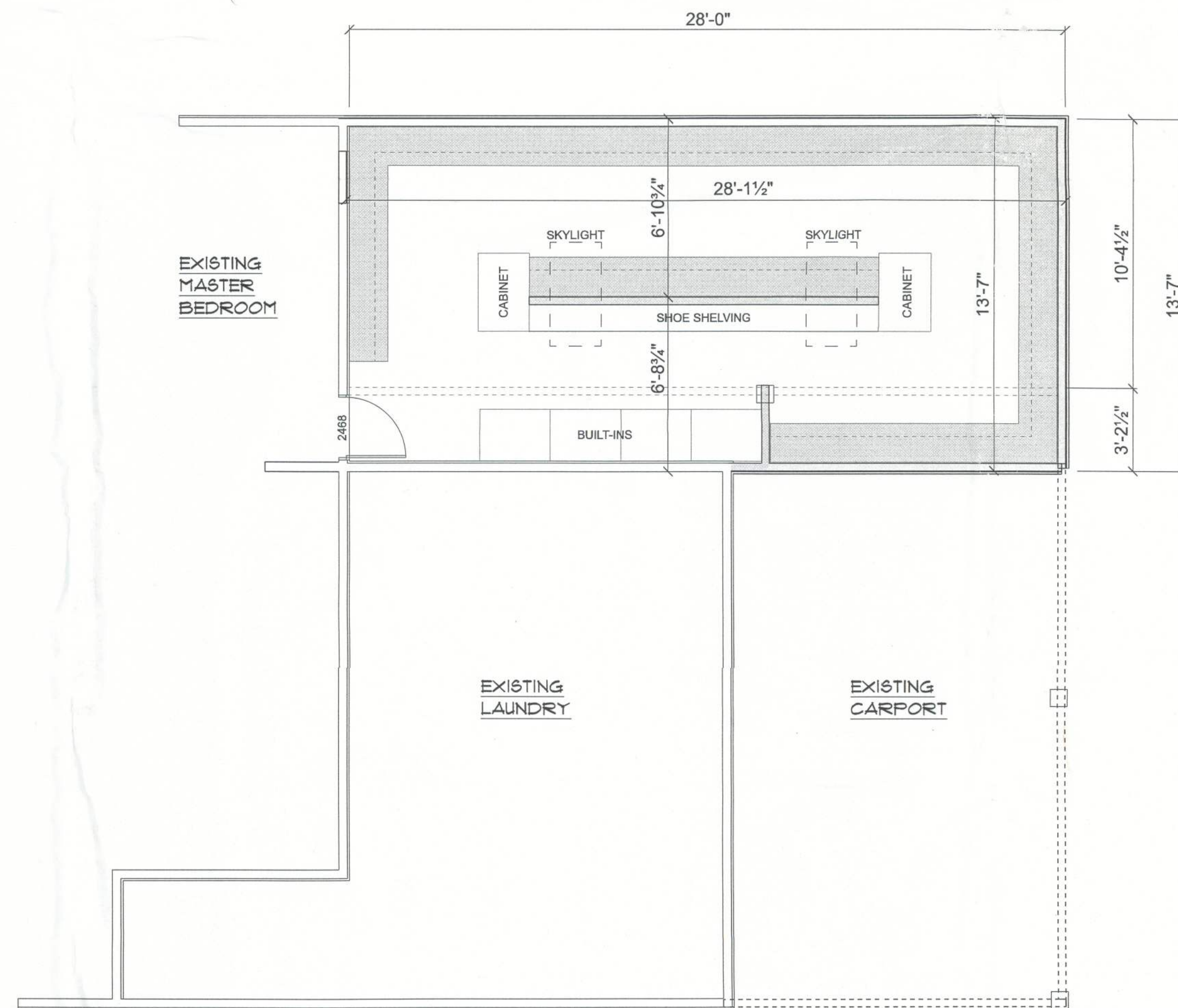
CLOSET ADDITION PLAN SCALE: 1/4" = 1'-0"
