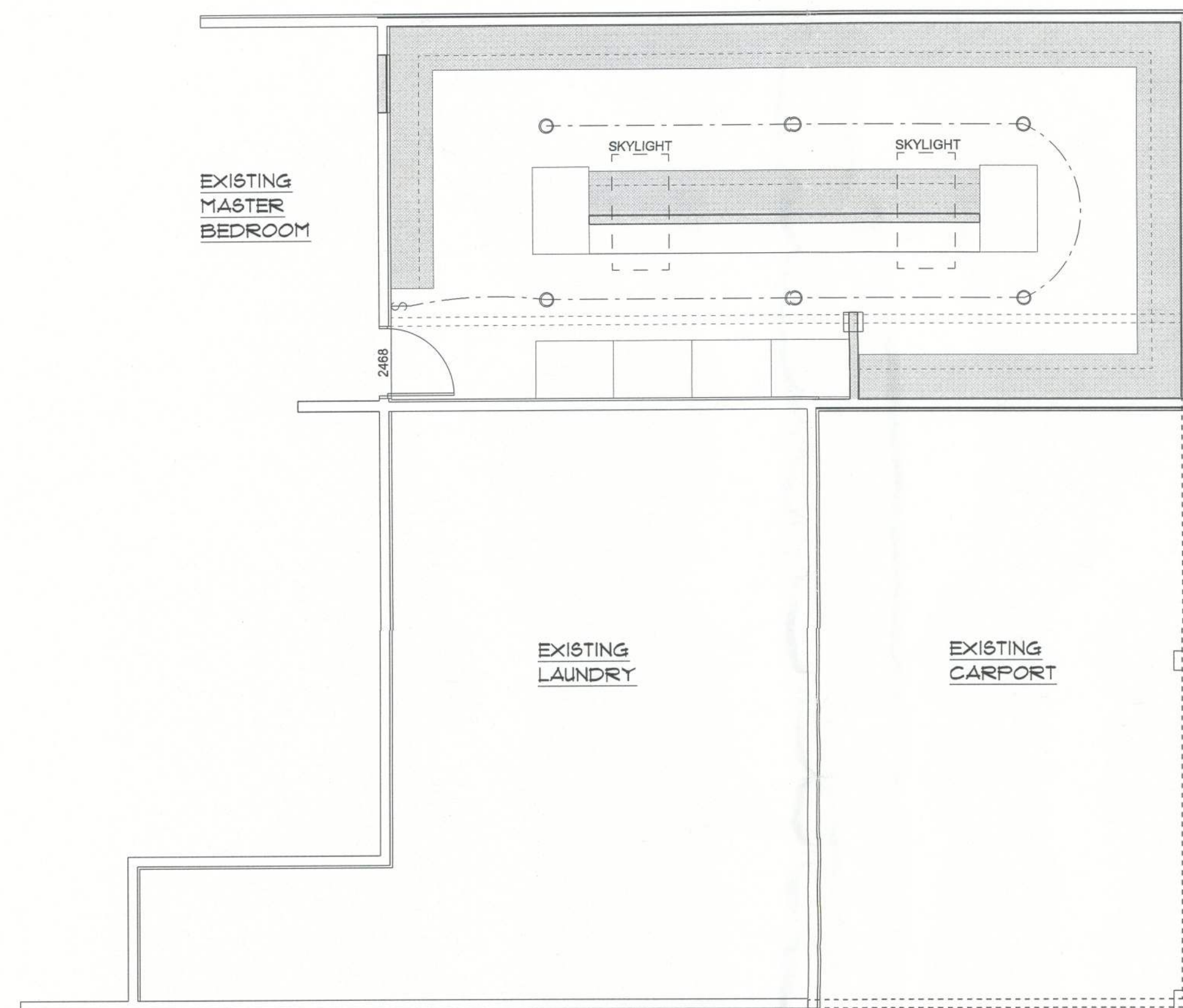
CLOSET ELECTRICAL PLAN SCALE: 1/4" = 1'-0"
