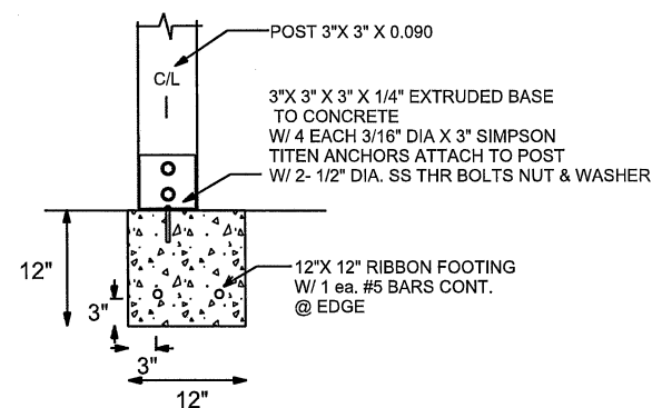
POST TO CONCRETE
