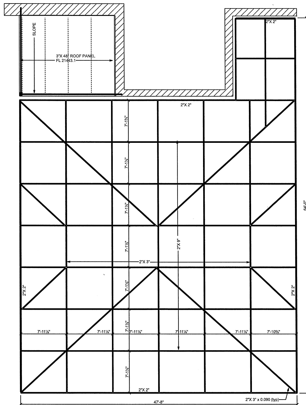
PLAN VIEW
