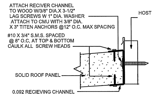
SOLID ROOF PANEL ATTACHMENT TO HOST NTS
