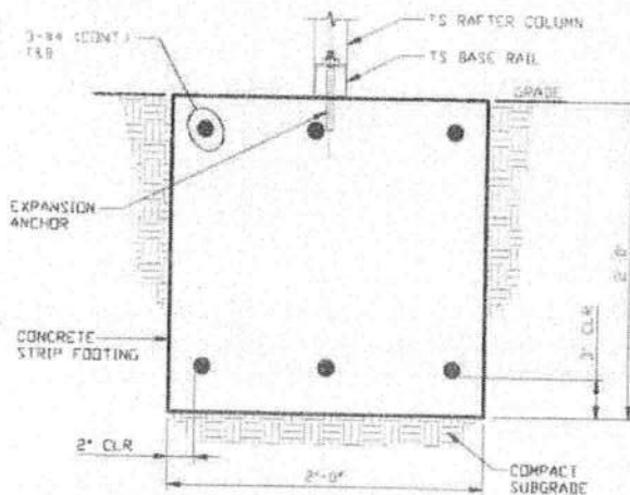
SECTION 1
