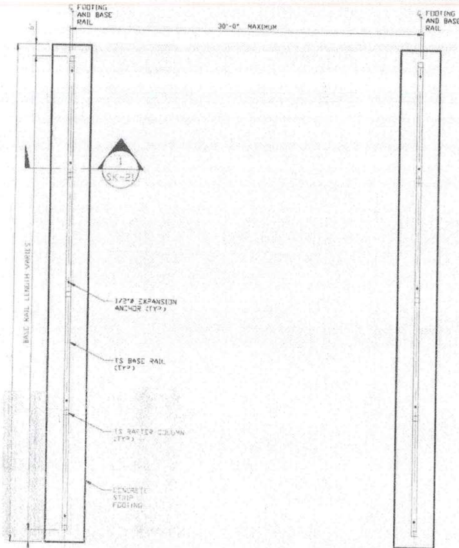
CONCRETE STRIP FOOTING PLAN
