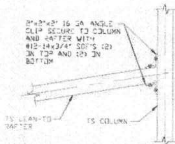
LEAN-TO RAFTER TO RAFTER COLUMN CONNECTION DETAIL FOR RAFTER SPANS < 15'-0"
