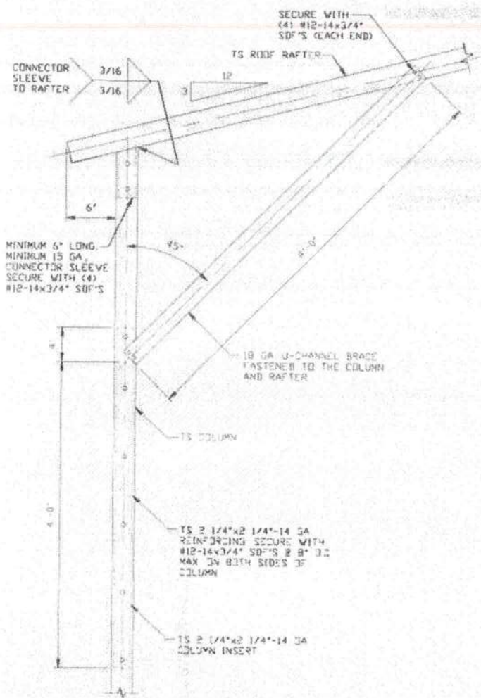
1A BOX EAVE RAFTER COLUMN CONNECTION DETAIL FOR HEIGHTS 10'-0" < TO ≤ 13'-0"
