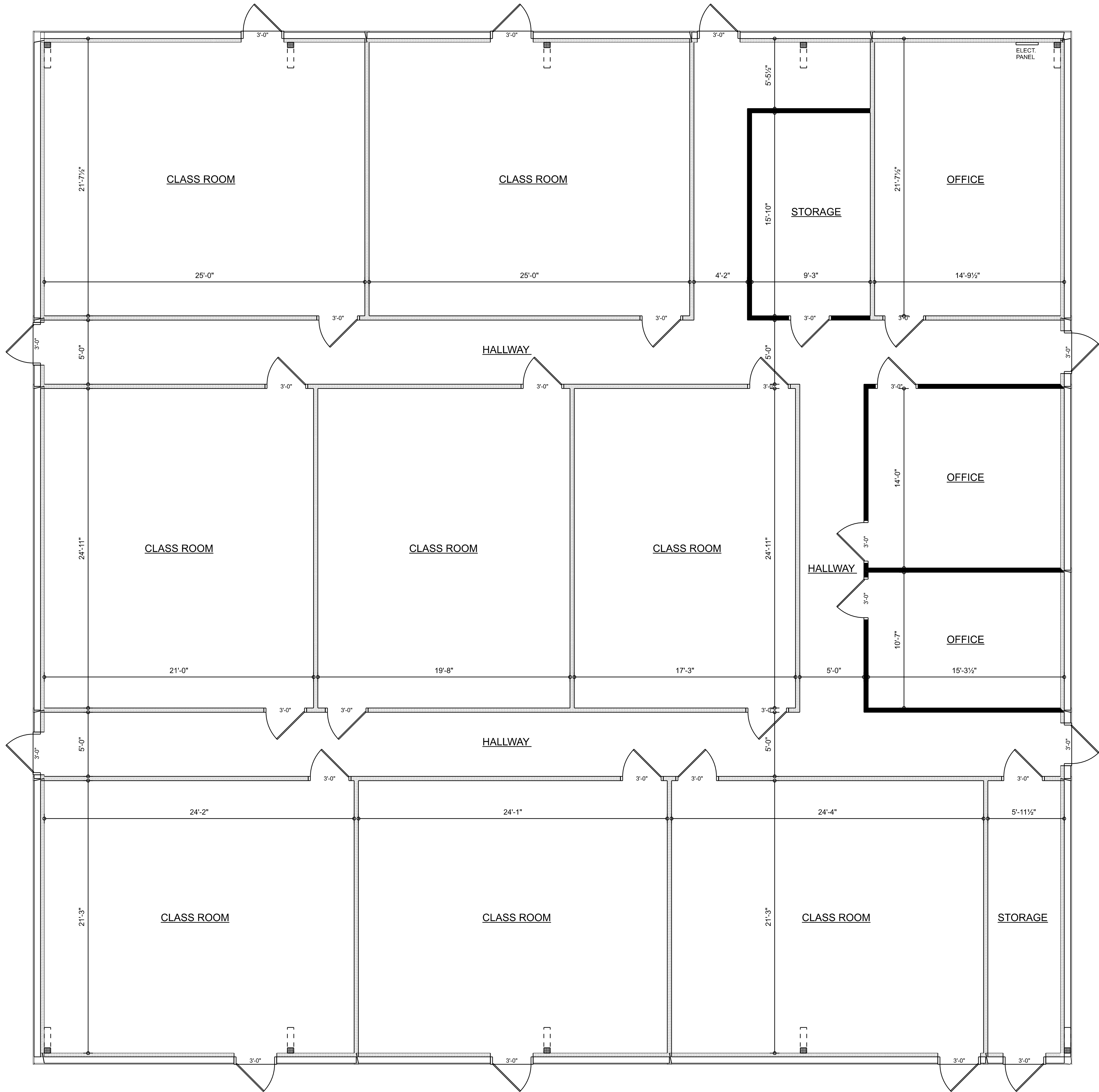
RENOVATED FLOOR PLAN SCALE: 1/4" = 1'-0"
